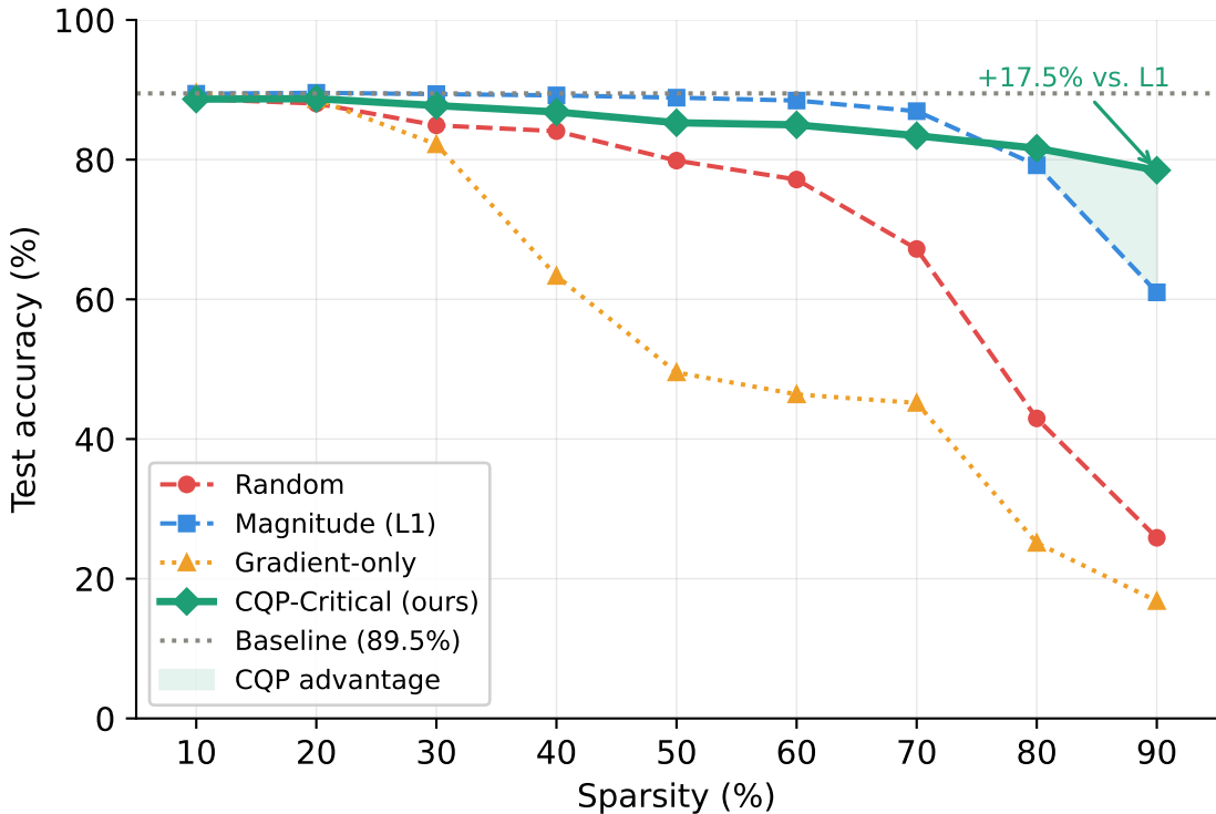
Accuracy-Sparsity Trade-off (fc1 layer, 4-method comparison)
